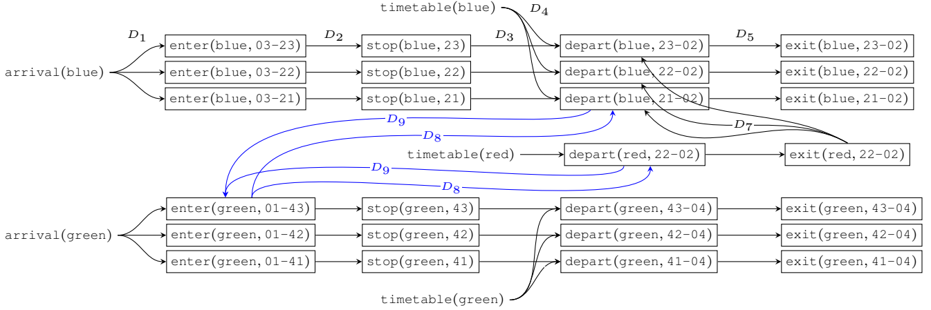
Figure 2: An example HDN N_X for the InStaDi task of Fig. 1. Boxed nodes represent actions in A . Black edges are the dependencies D_1 to D_7 . Blue edges are the dependencies D_8 to D_{11} . To avoid visual clutter, not all blue dependencies are drawn.
