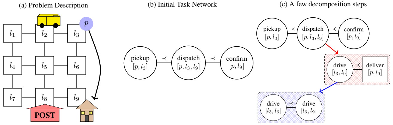
Figure 1: (a) Deliver package P to someone at location 9 who may or may not be at home with an equal probability. In case they are not at home, the package must be delivered to the post office. (b) The initial task network consisting of three compound tasks. (c) A few steps of decomposing the initial task network into a more refined one. By convention, primitive tasks are square and compound ones are circular.
