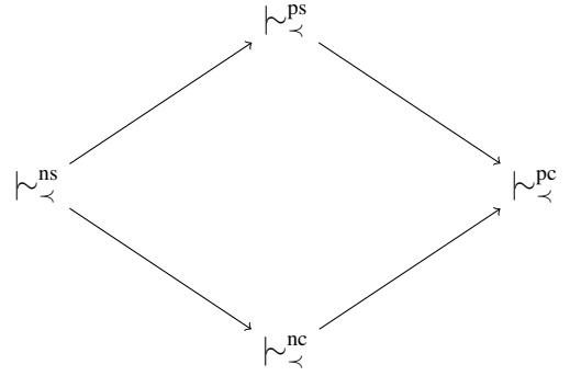
Figure 2: Relationship among \sim_{\prec}^{ns} , \sim_{\prec}^{nc} , \sim_{\prec}^{ps} , \sim_{\prec}^{pc} for an arbitrary \prec , given that \prec is well-founded. Arrow directions indicate the antecedent to consequent relation.
