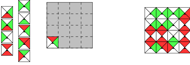
Figure 5: A set of tile types and an empty square, and a solution.
