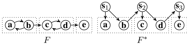
Figure 7: Independence of b and e given c not derivable
